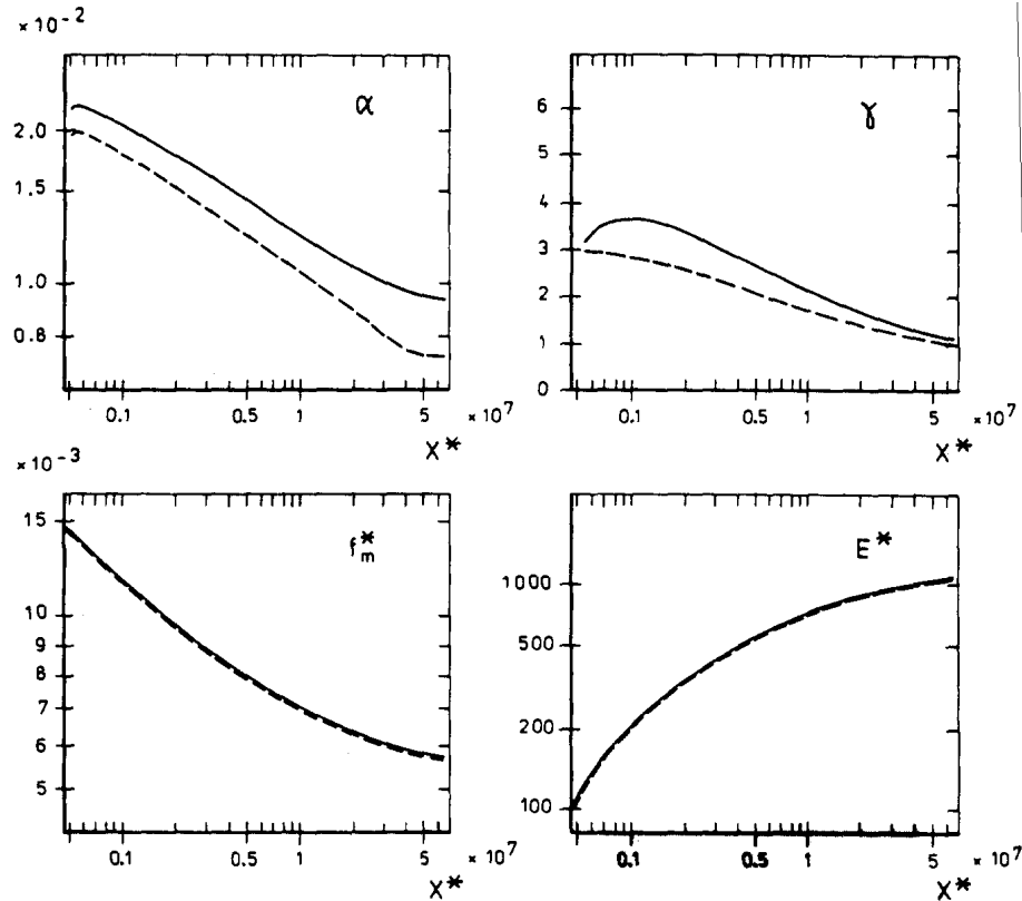
Figure 3.5 Comparison of fetch-growth curves for spectral parameters computed using the exact form and the discrete interaction approximation of S_{nl} . All variables are made dimensionless using u_* and g .
