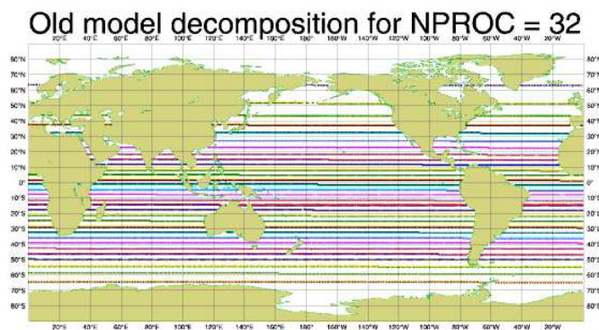
Figure 6.4 1-D decomposition of the WAM model 0.5 \times 0.5 irregular lat-long grid for 32 processors. The different colour lines indicate grid points sharing information with neighbouring PEs.
