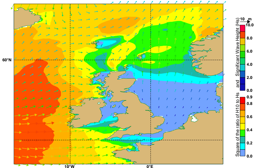
Figure 10.6 Square of the ratio of H_{10} to H_s (colour shading), Significant Wave Height ( H_s ) (arrow length and colour) on 23 March 2016, 6 UTC.
