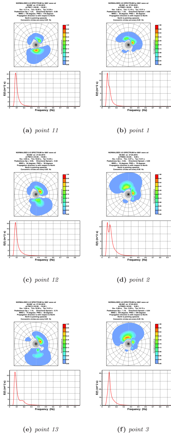
Figure 10.1 Normalised 2d spectra (top of each panel) and frequency spectra (bottom of each panel) on 23 March 2016, 6 UTC, for locations shown in Figure 10.3. The 2-D spectra were normalised by their respective maximum value. The concentric circles in the polar plots are spaced every 0.05 Hz
