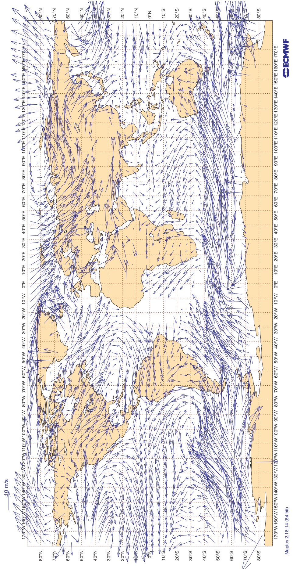
Figure 14 ECMWF Monitoring Statistics: Apr 2014 AMV Winds: 700-1000hPa Mean Observed Wind
