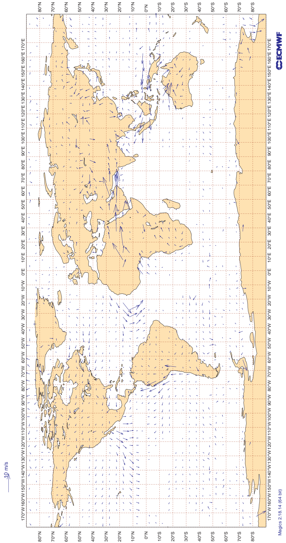
Figure 16 ECMWF Monitoring Statistics: Apr 2014 AMV Winds: 700-1000hPa Wind bias: Observation - FG
