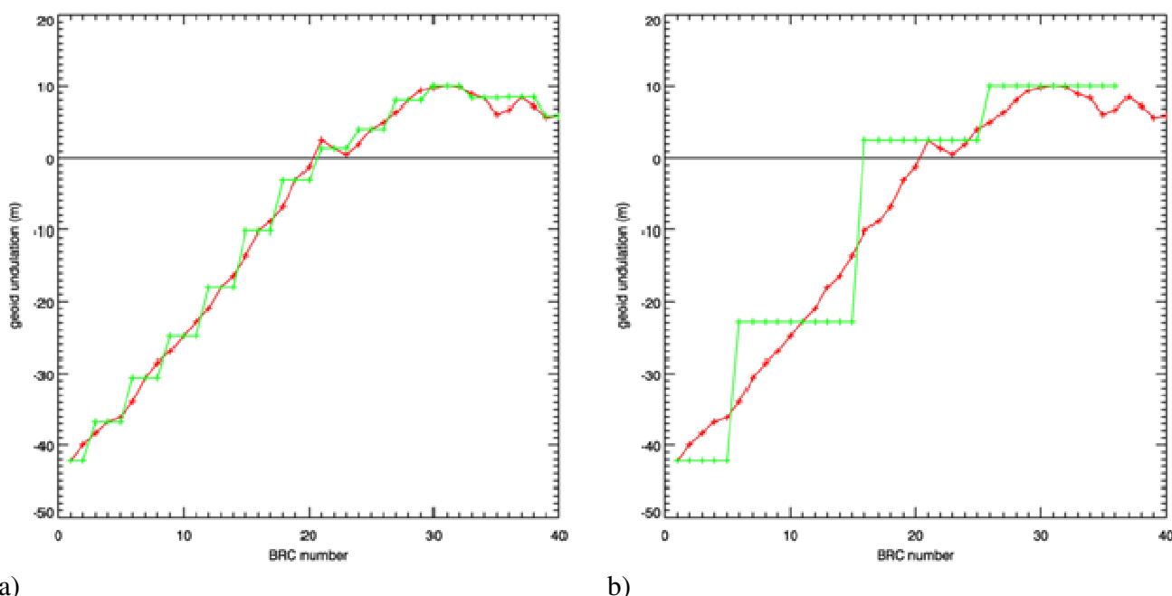
Figure 16. The geoid height is plotted as a function of BRC number (from L1B data) in red. In green shows what effectively happens with the grouping algorithm, in that the central index of the observation value is applied. In a) the grouping is set to 3 BRCs, in b) the grouping is set to 10 BRCs.
