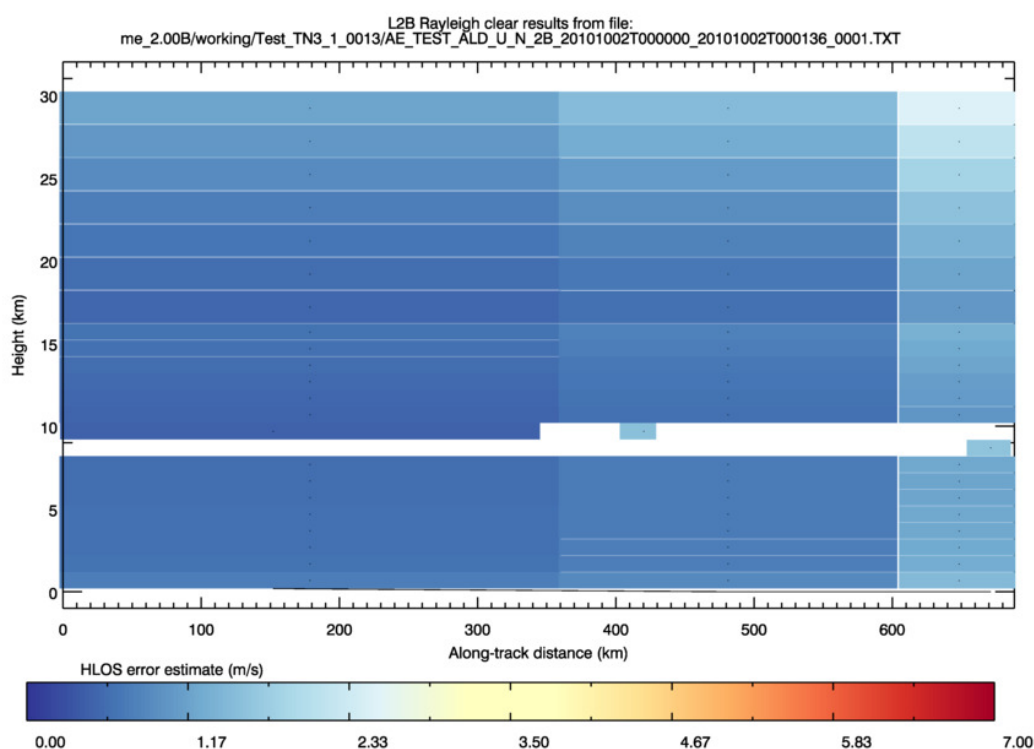
Figure 15. Estimated Rayleigh-clear HLOS standard error (m/s) as produced by the L2B processor for the test case of Figure 14.
