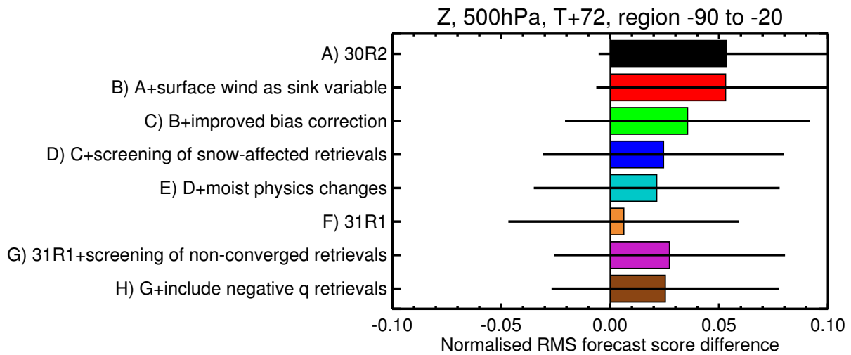
Figure 2: Normalised difference in RMSE forecast verification score for geopotential height at 500hPa, for the month of August 2005, taking the difference between experiments A to H (containing rainy SSM/I observations) and the control experiment X, from which rainy observations have been excluded. Forecast scores are based on the RMS difference between southern hemisphere T+72 forecasts and own analysis of geopotential height at 500hPa, for the month of August 2005. Positive differences in RMSE indicate a degradation in the experiment compared to the control; negative differences show an improvement. Error bars indicate the 90% confidence range for a significant difference between experiment and control.
