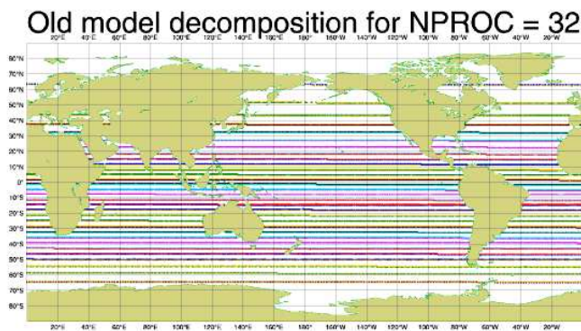
Figure 6.4 1-D decomposition of the WAM model 0.5 \times 0.5 irregular lat-long grid for 32 processors. The different colour lines indicate grid points sharing information with neighbouring PEs.
