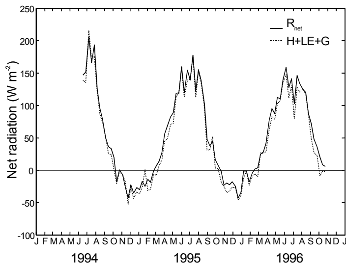
Figure 2: Measured net radiation and sum of measured sensible, latent and ground heat flux (10-days average).
