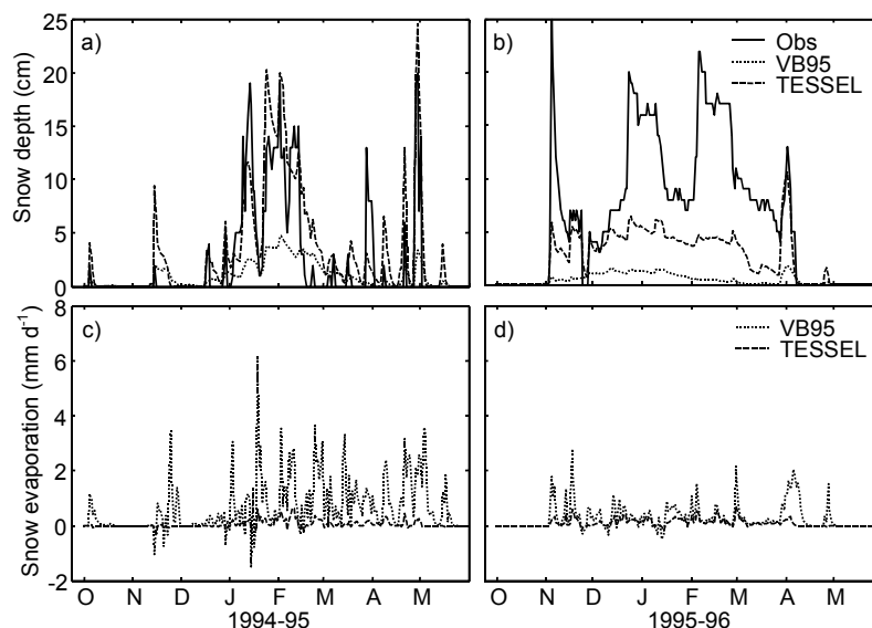
Figure 8: a-b) Simulated and measured (Uppsala Airport) snow depth, and c-d) simulated snow evaporation, winter 1994-95 and winter 1995-96.
