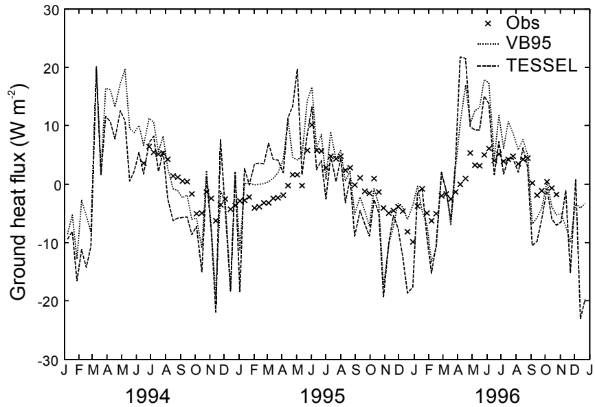
Figure 6: Simulated and measured ground heat flux (10-day averages).
