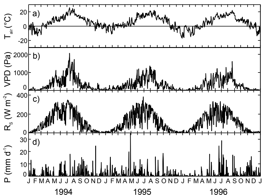
Figure 3: Weather conditions during the three years of simulation: a) air temperature, b) vapor pressure deficit, c) global radiation, and d) precipitation (daily average values).
