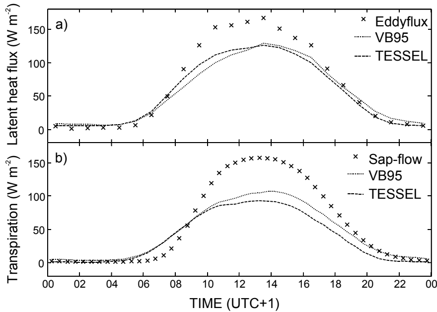
Figure 13: a) Simulated and measured latent heat flux and b) simulated transpiration and observed sap flow, average diurnal course 4 July-31 August 1995.
