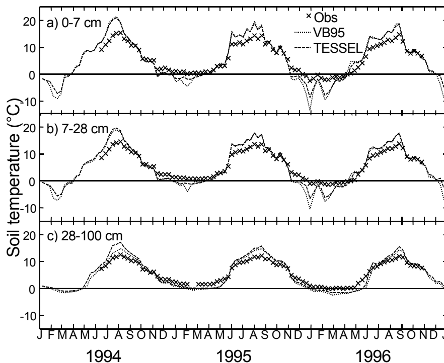
Figure 10: Simulated and measured soil temperature in model layers at a) 0-7 cm, b) 7-28 cm and c) 28-100 cm (10-days averages). Measurements from 15 soil profiles were averaged and integrated over the model layer depths to represent the simulations.
