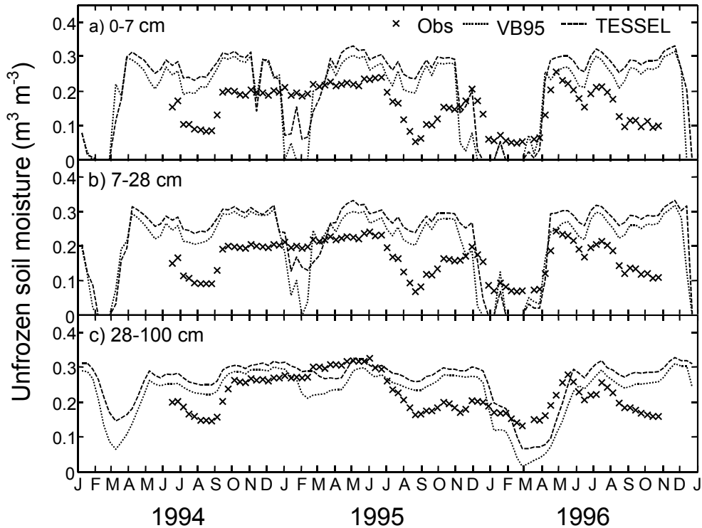
Figure 11: Simulated and measured unfrozen soil moisture in model layers at a) 0-7 cm, b) 7-28 cm, and c) 28-100 cm (10-days averages). Measurements from 15 soil profiles were averaged and integrated over the model layer depths to represent the simulations.
