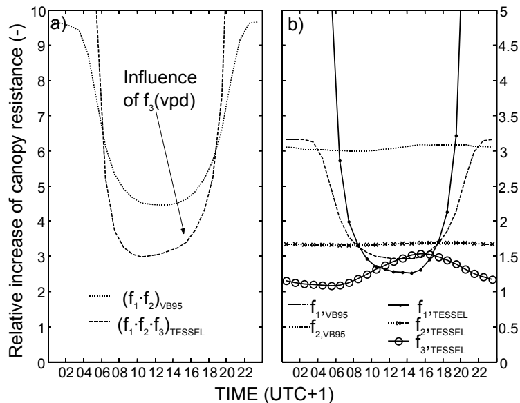
Figure 14: a) Relative increase of canopy resistance in the VB95 and TESSEL simulations, and b) their components representing stress due to solar radiation ( f_1 ), soil moisture stress ( f_2 ) and vapor pressure deficit ( f_3 ), average diurnal course 4 July-31 August 1995.
