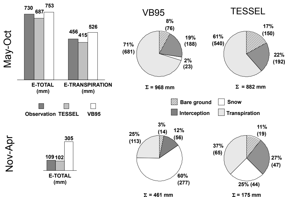
Figure 15: Left: Total evaporation and transpiration simulated by the VB95 and TESSEL models and observed with eddy-correlation (E-total) and sap flow (E-transpiration), based on 435 days May-Oct and 358 days Nov-Apr 1994, 1995 and 1996. Right: Evaporation from different components simulated by the VB95 and TESSEL models, based on 552 days May-Oct and 543 days Nov-Apr 1994, 1995 and 1996.
