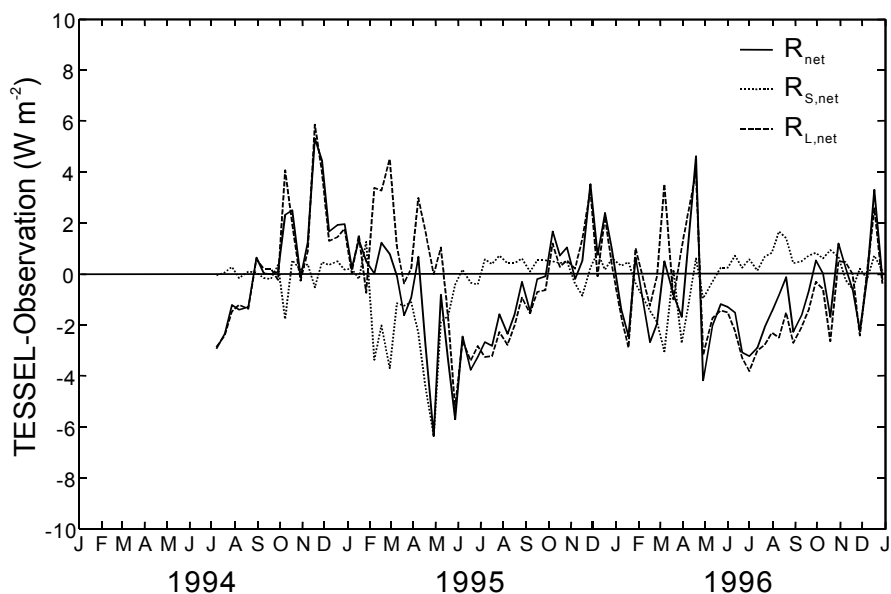
Figure 7: Discrepancy between simulated (TESSEL) and measured net shortwave radiation, net longwave radiation, and net radiation (10-day averages).
