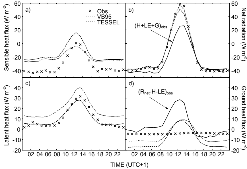
Figure 9: Surface heat fluxes (turbulent fluxes of sensible and latent heat are positive upwards, net radiation and ground heat flux are positive downwards), average diurnal course October-December 1995.
