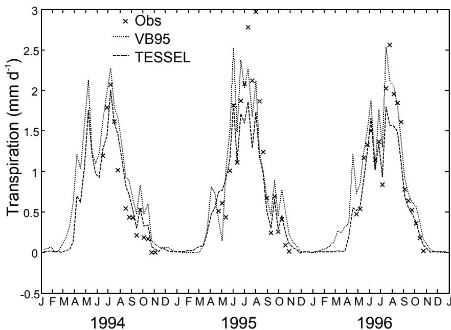
Figure 12: Simulated transpiration and measured sap flow (10-day averages).
