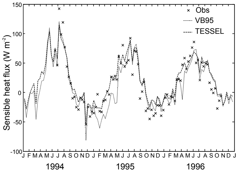
Figure 5: Simulated and measured sensible heat flux (10-day averages).
