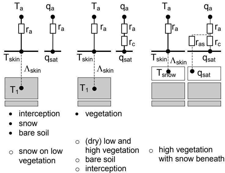
Figure 1: Resistance scheme for three types of coupling between the surface and the atmosphere (from van den Hurk et al, 2000). The list below each scheme refers to the sub-grid fraction types (tiles) in the VB95 (black dots) and the TESSEL (circles) models.
