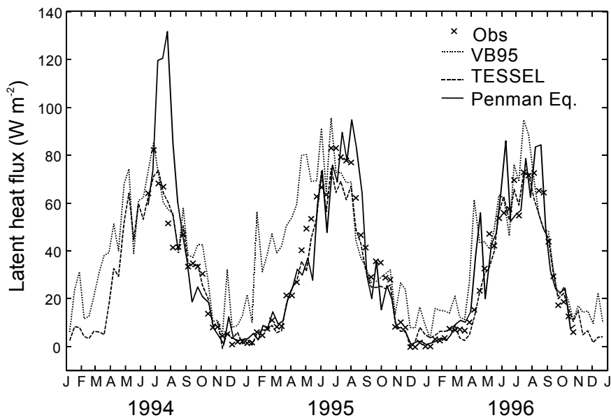
Figure 4: Simulated and measured latent heat flux (10-day averages).
