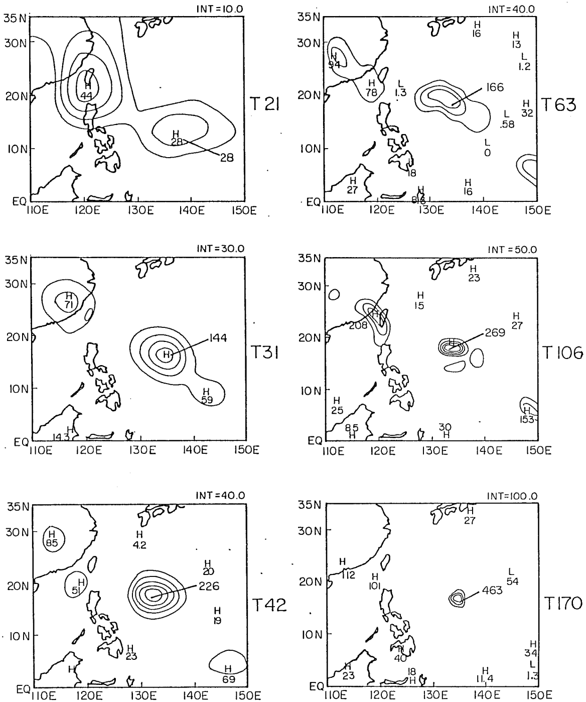
Fig. 11b Geographic distribution of rainfall accumulated between 48 and 72 hours.
