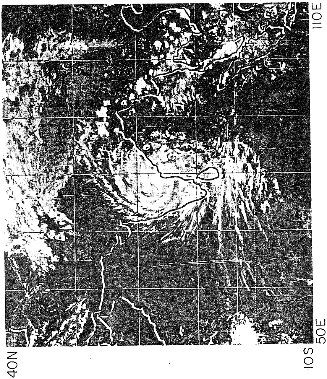
Fig. 6b Satellite imagery (DMSP); May 12, 1979, 12 UTC
