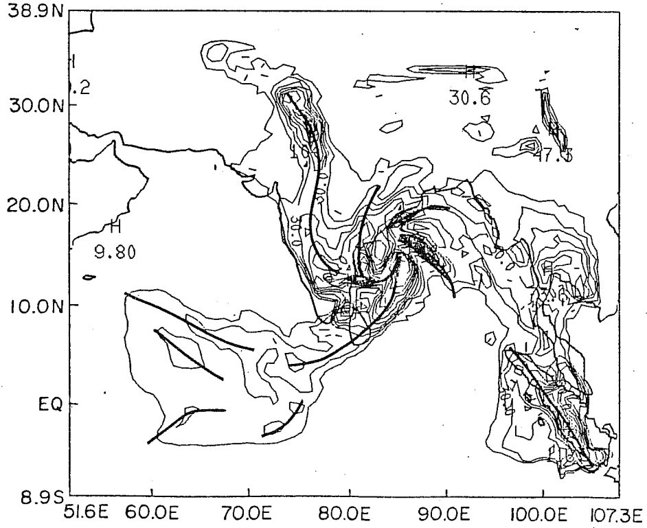
Fig. 7a Predicted rainfall hours 0 to 24, mm/day.
